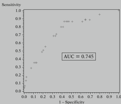
ROC plot
